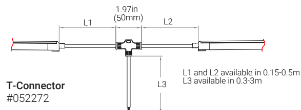
Extension #052270
