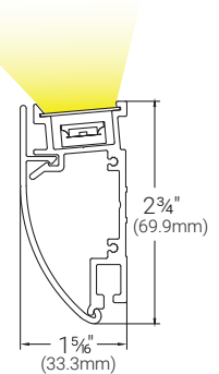
Uplight - Profile View
