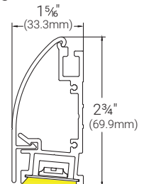
Downlight - Profile View
