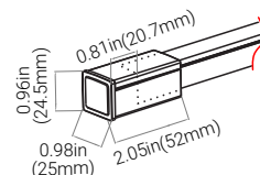
Snap End Cap #052236S
