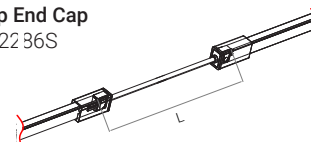
Snap Extension RGB #052274S-CU16 RGBW #052275S-CU16 L available in 0.3m, 1m, 3m
