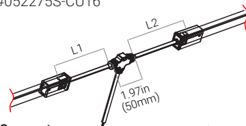
Snap T-Connector RGB #052276S-CU16 RGBW #052277S-CU16 L1 and L2 available in 0.3m
