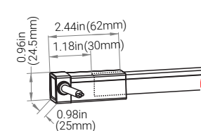
Side Feed Snap Connector, 16'L RGB #052254S-CU16 RGBW #052261S-CU16
