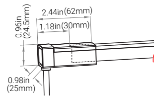
Bottom Snap Connector, 16'L RGB #052253S-CU16 RGBW #052260S-CU16
