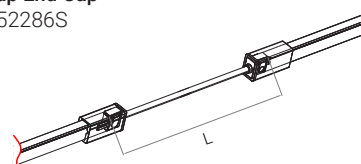
Snap Extension #052270S L available in 0.3m, 1m, 3m
