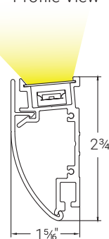
Uplight - Profile View
