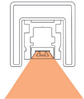
Full cut-off
