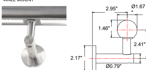
WALL MOUNT
