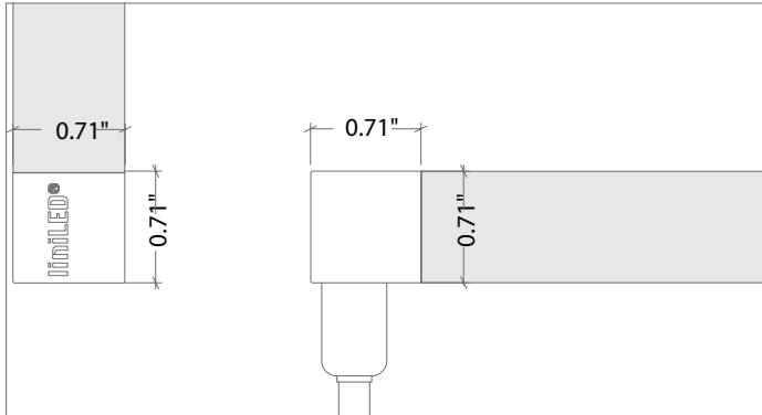
OrgaLED® Diffuse Connector 90° Angle 3/4"
