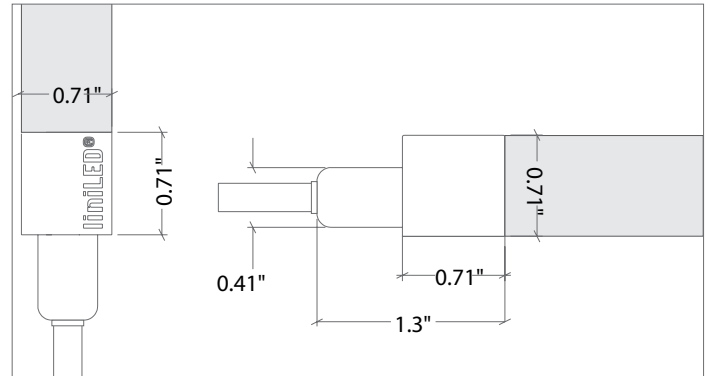
OrgaLED® Diffuse Connector Straight 3/4"
