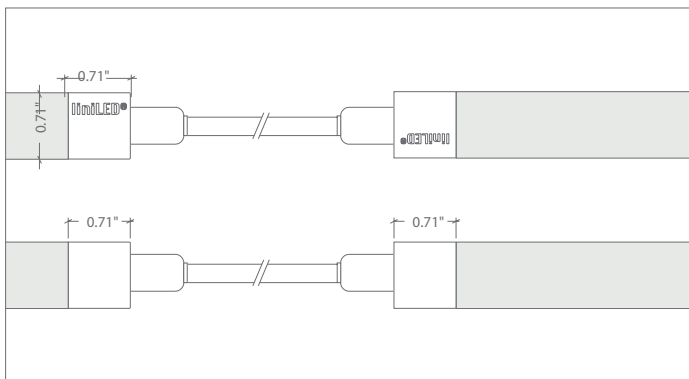
OrgaLED® Diffuse Extension Cord 3/4"
