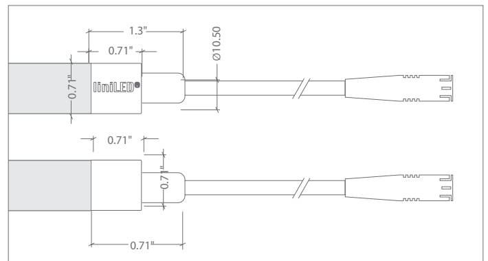
OrgaLED® Diffuse Connector Male/Female 3/4"
